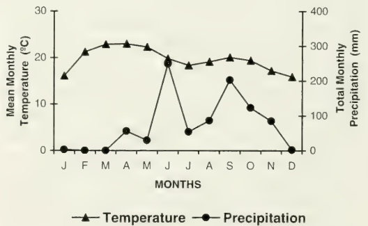
Fig. 2. Monthly abundances of individuals of Onthophagus chevrolati retusus (Scarabaeinae) and Onthotrupes viridiobscurus (Geotrupinae) found in samples of cow and horse dung from El Llano de las Flores, Oaxaca, January–December 2003; and mean monthly temperature and total monthly precipitation (data taken from the climatological station of San Juan de Atepec, Oaxaca, provided by the National Water Commission).
